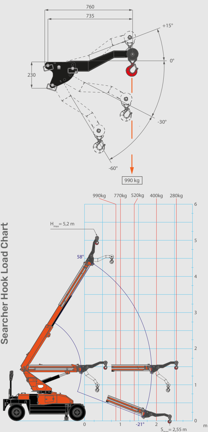
Hook Load Chart
